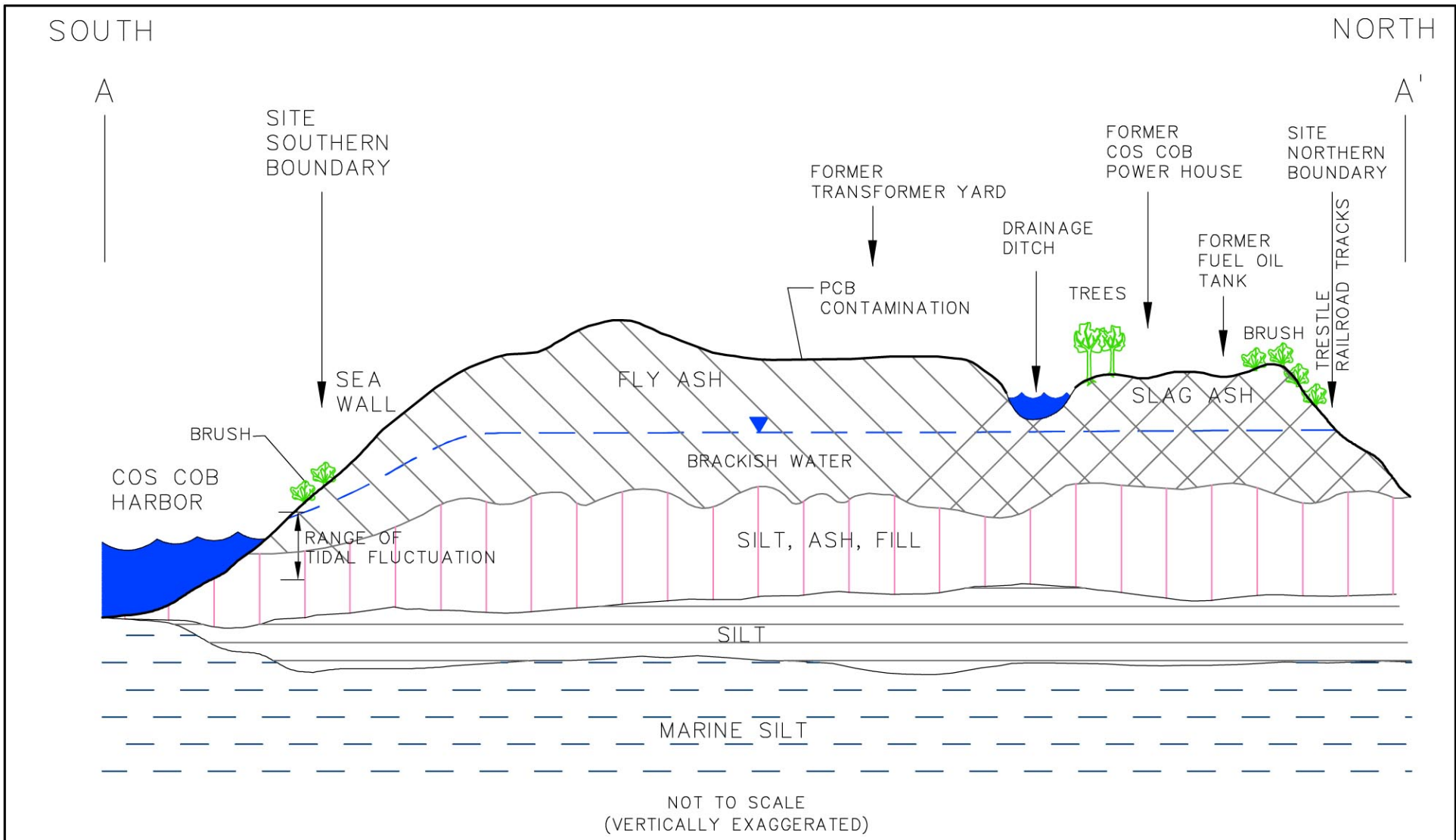
FORMER COS COB POWER PLANT GREENWICH, CONNECTICUT FIGURE 2 CONCEPTUAL SITE MODEL DIAGRAM U.S. EPA REGION I IN COOPERATION WITH BROWNFIELDS TECHNOLOGY SUPPORT CENTER
