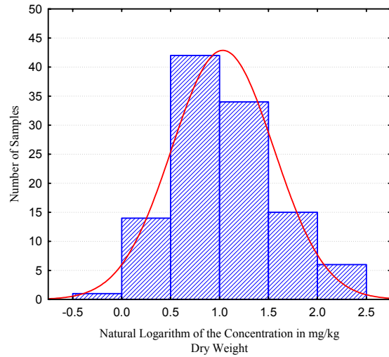
Histogram Logtransformed Data Arsenic Fixed Laboratory Results on a Dry Weight Basis K-S d=.12765, p<.10 ; Lilliefors p<.01 Shapiro-Wilk W=.95317, p=.00062
