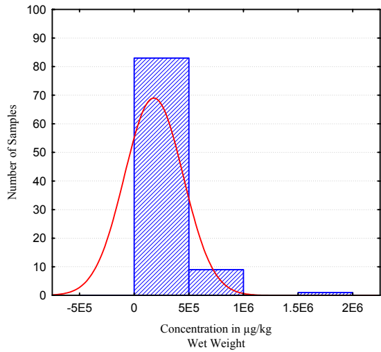
Histogram Untransformed Data Total PAHs Site Lab Field Test Kit Results on a Wet Weight Basis K-S d=.25179, p<.01 ; Lilliefors p<.01 Shapiro-Wilk W=.63605, p=.00000
