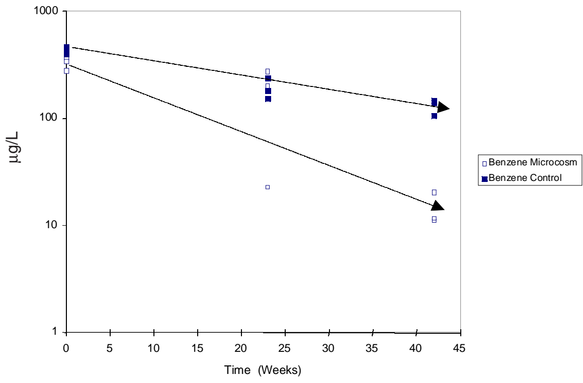
Figure C.3.12 Benzene microcosm results.
