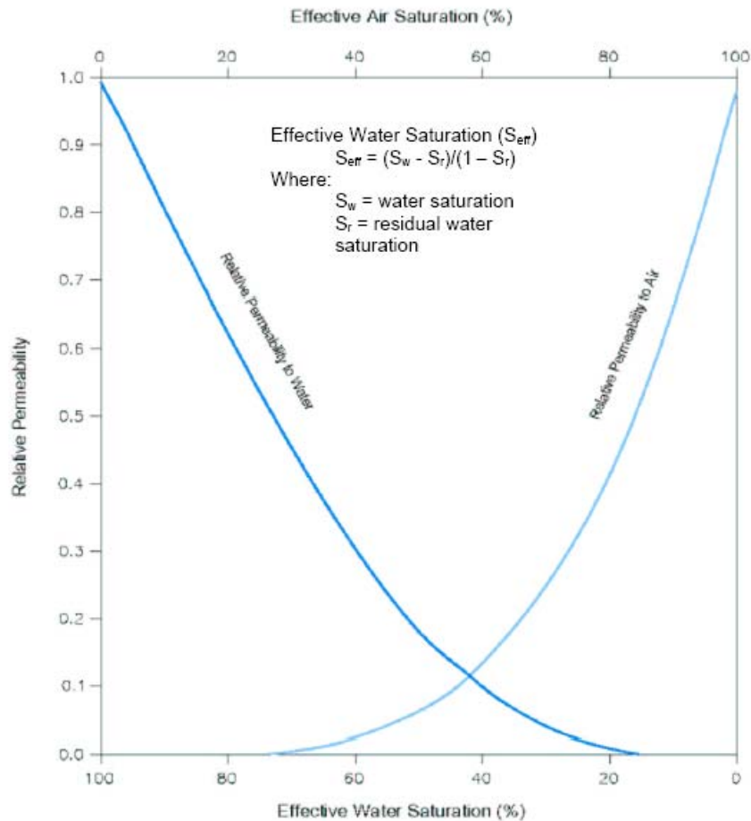
Figure 2-13. Typical Relationship of Relative Permeability and Saturation, in a Soil Partially Saturated with Air and Water. As the water saturation increases, the relative permeability of the soil with respect to water increases, but the relative permeability to air decreases.
