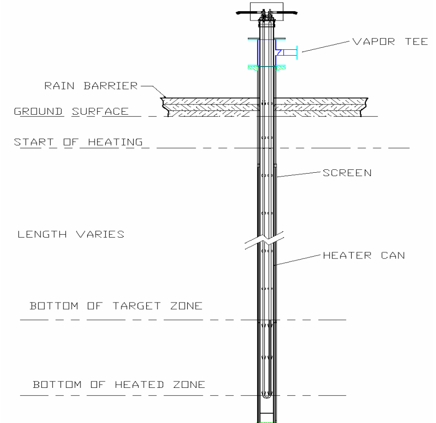
Figure 6-4. Typical Producer Well.
