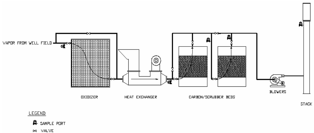
Figure 5-3. Typical Thermal Conduction Pilot-Test Process Diagram.
