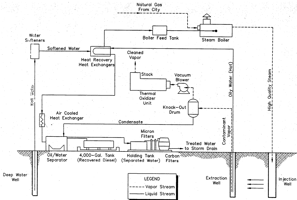
Figure 6-7. Typical Steam Injection System.
