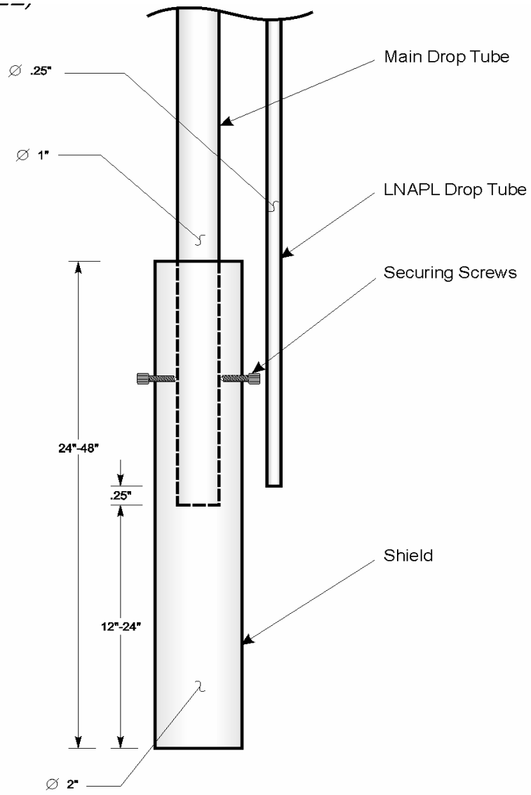
Figure 5. Engineering Design of the Dual Drop Tube System
